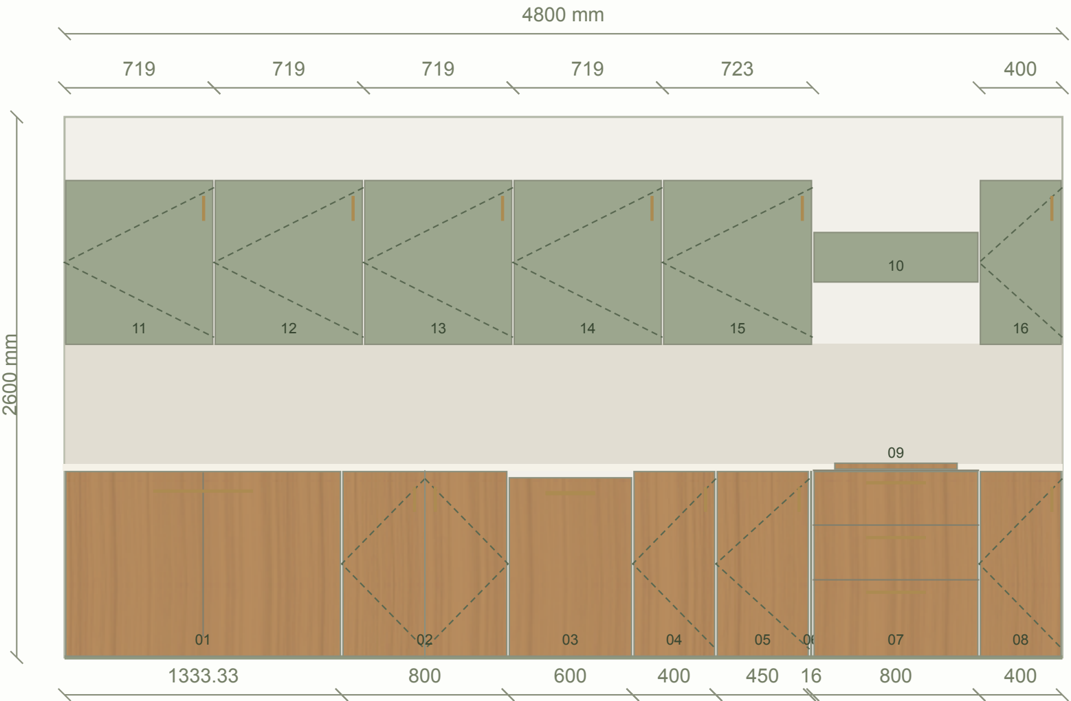
WALL A · FRONT ELEVATION
