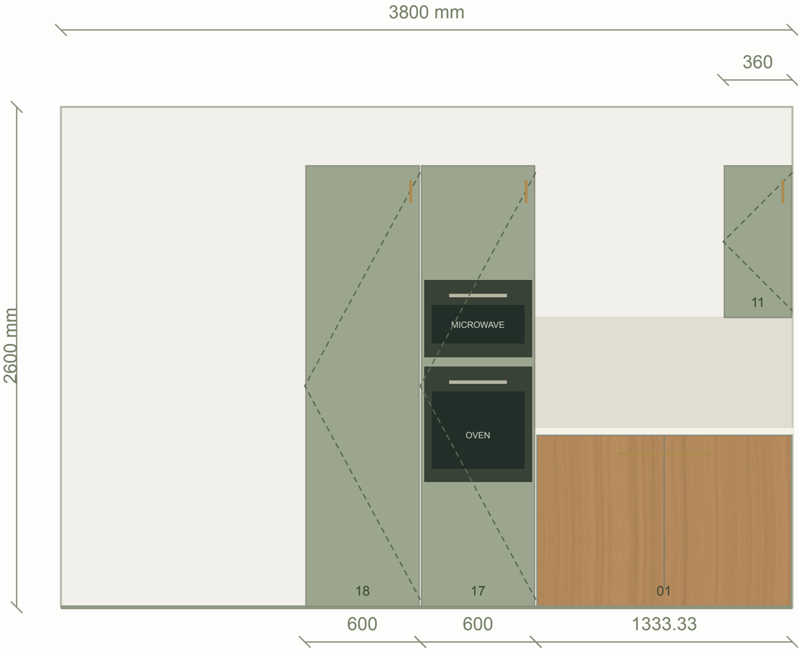
WALL D · FRONT ELEVATION
